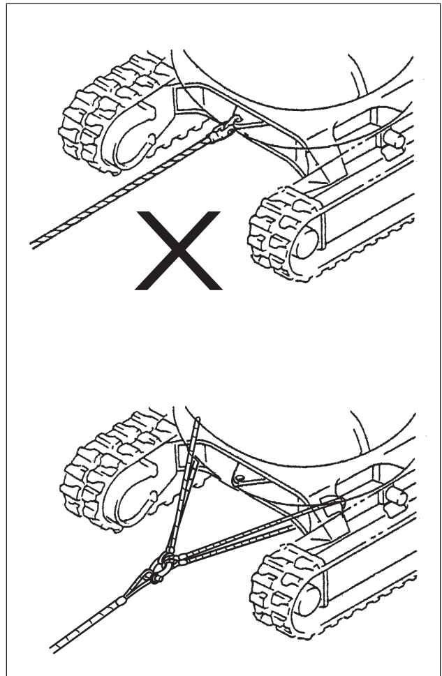
Fig. 2-2 TOW MACHINE PROPERLY
